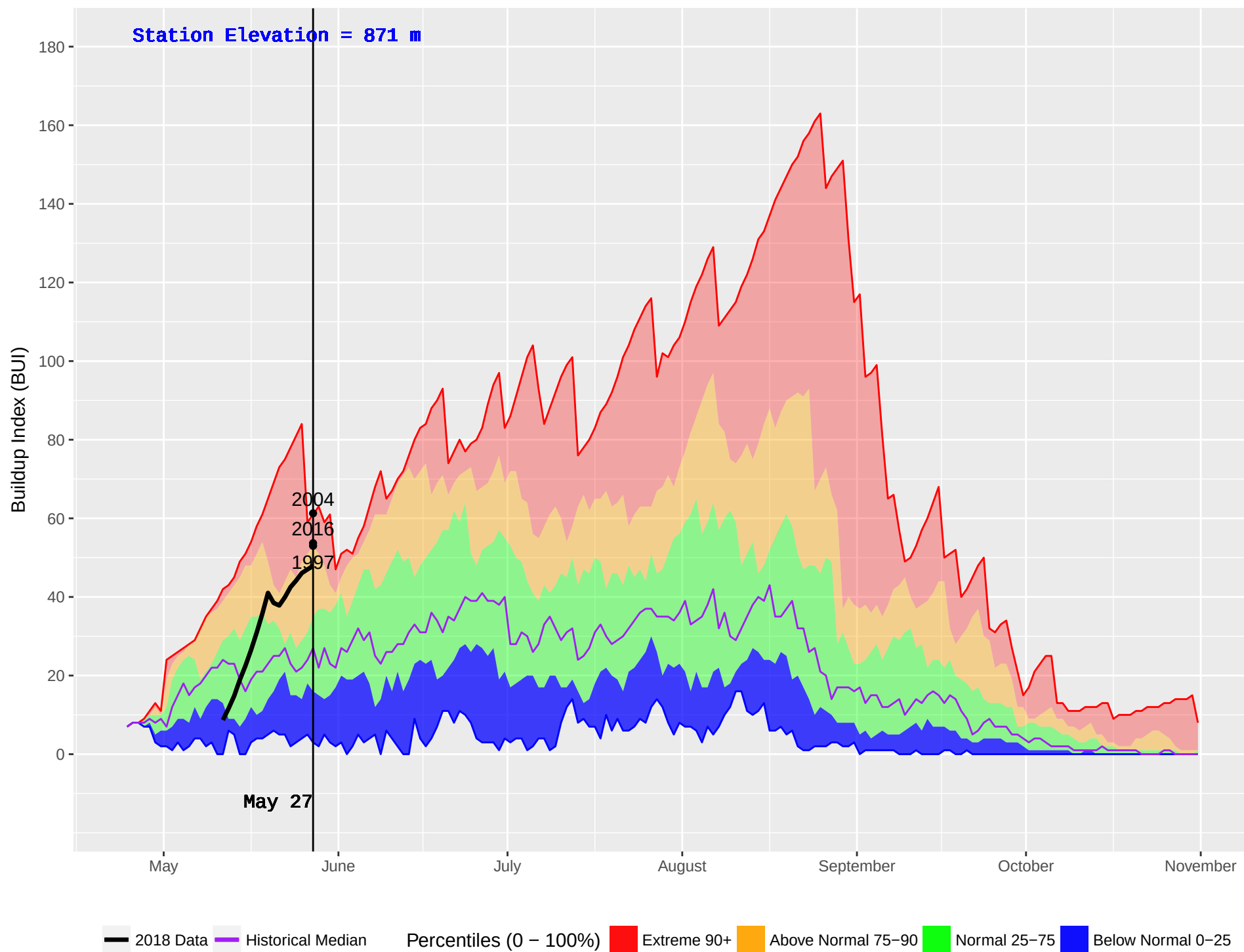
SUSTUT (156) : Historical (1989–2016) and Current (2018) Noon Buildup Index (BUI)
