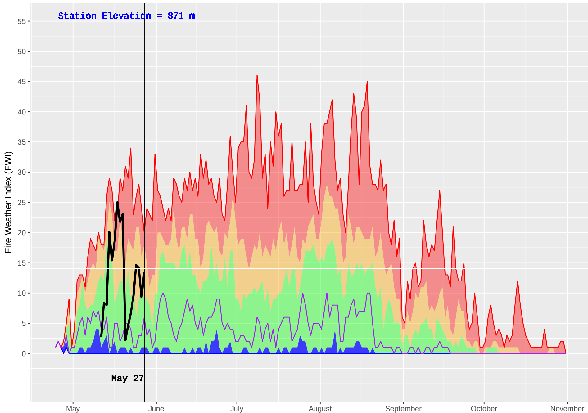
SUSTUT (156) : Historical (1989–2016) and Current (2018) Noon Fire Weather Index (FWI)
