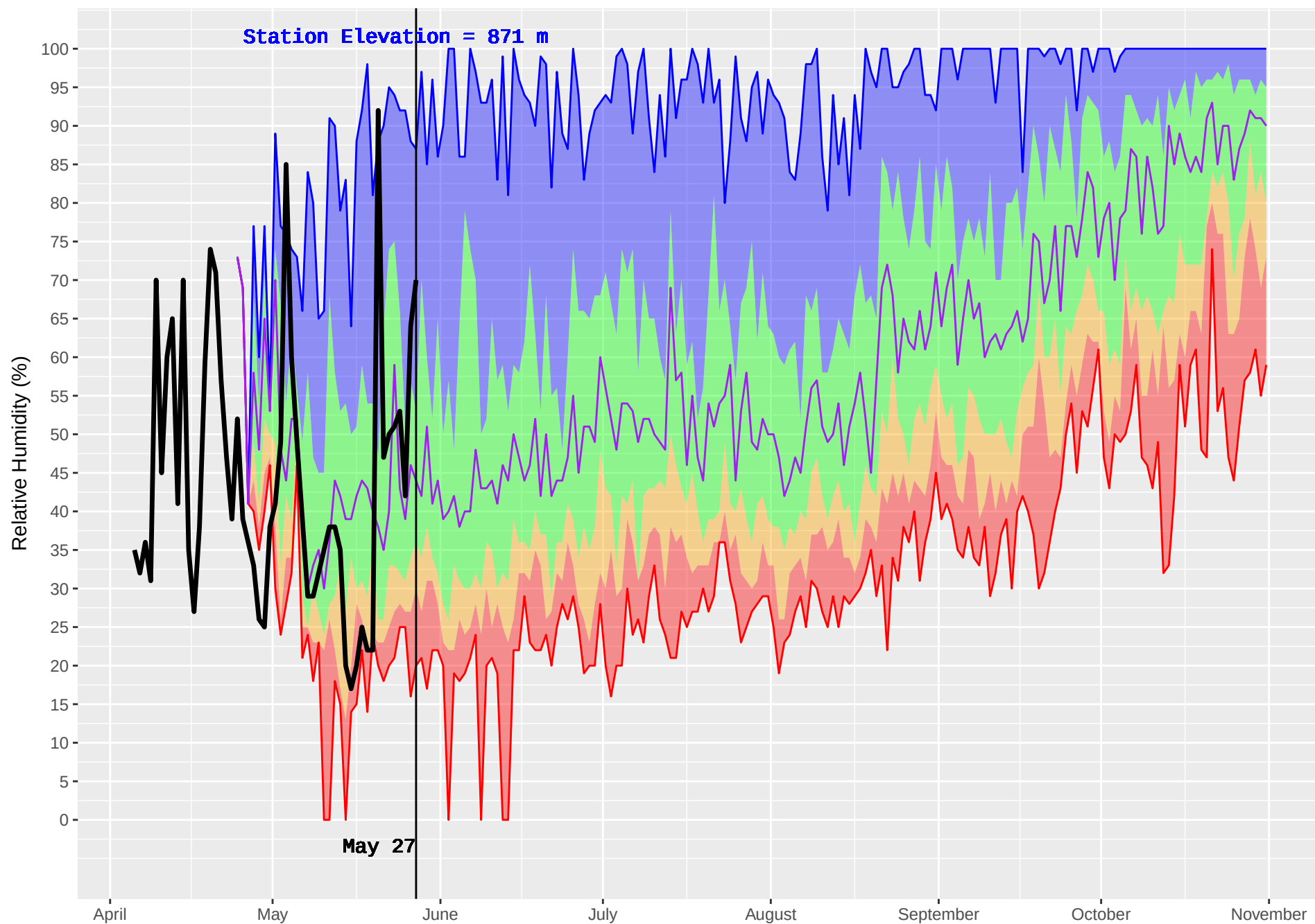
SUSTUT (156) : Historical (1989–2016) and Current (2018) Noon Relative Humidity
