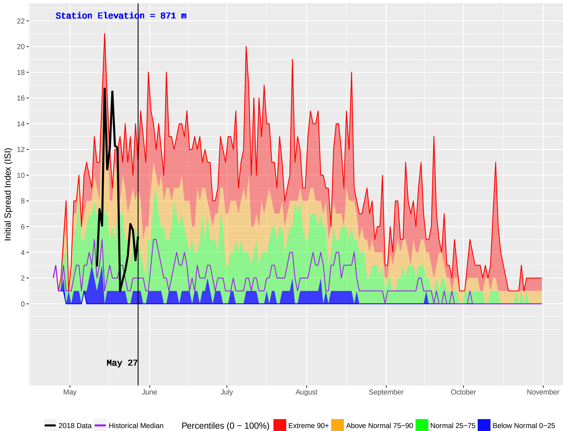
SUSTUT (156) : Historical (1989–2016) and Current (2018) Noon Initial Spread Index (ISI)
