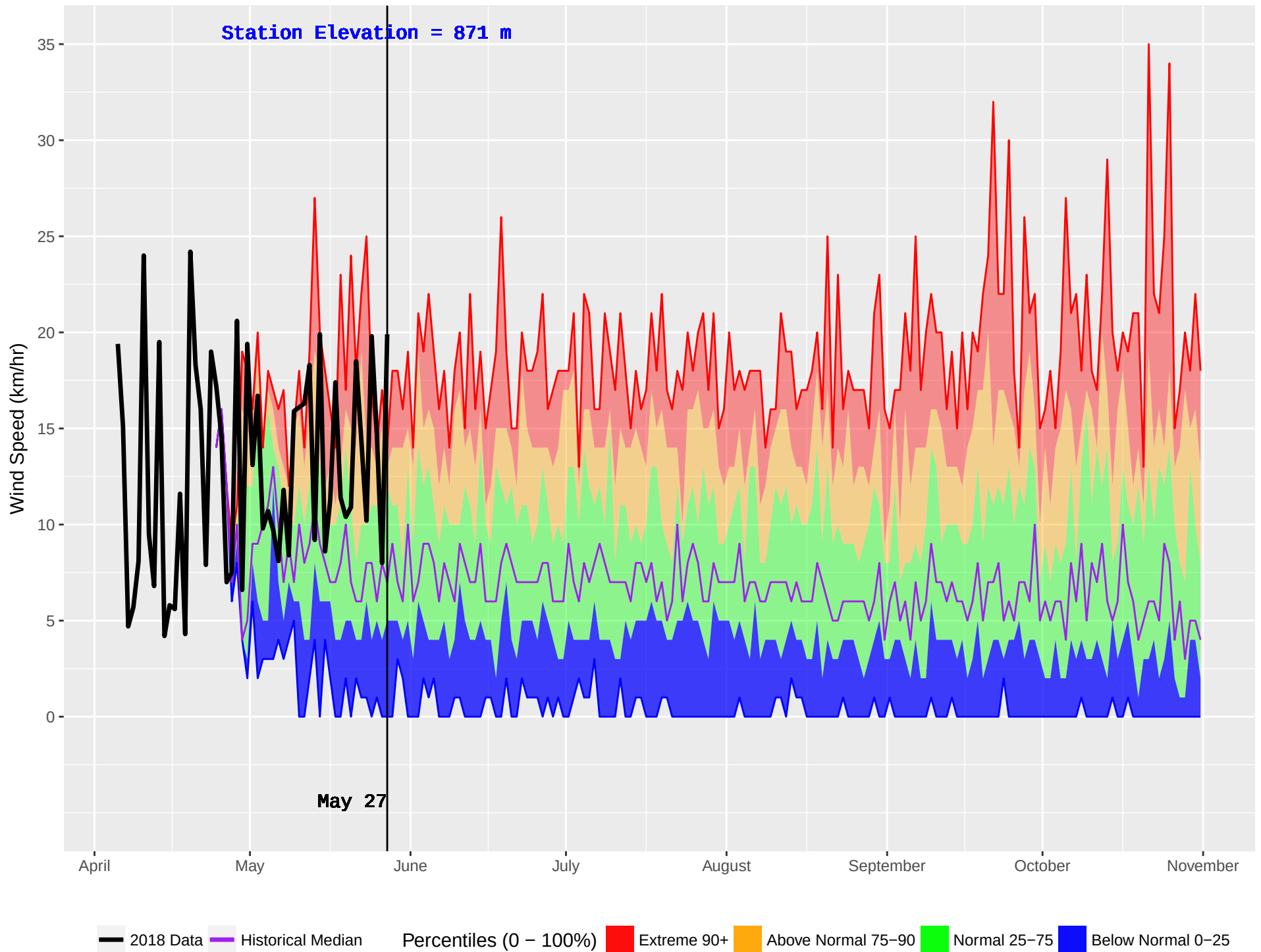
SUSTUT (156) : Historical (1989–2016) and Current (2018) Noon Wind Speed
