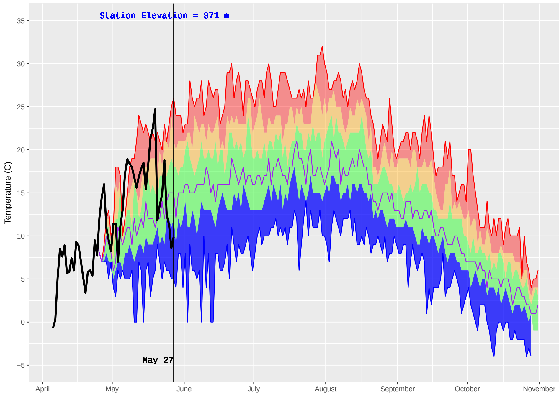
SUSTUT (156) : Historical (1989–2016) and Current (2018) Noon Temperature
