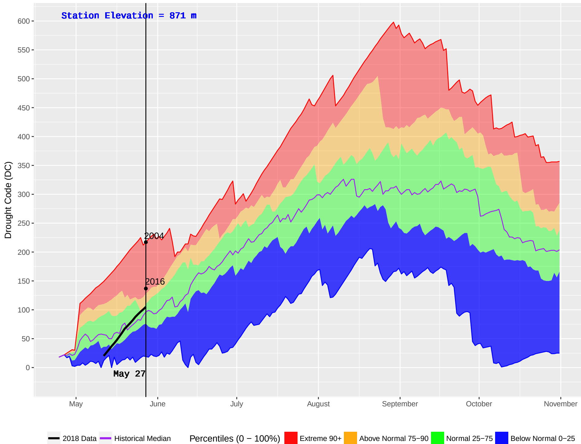
SUSTUT (156) : Historical (1989–2016) and Current (2018) Noon Drought Code (DC)
